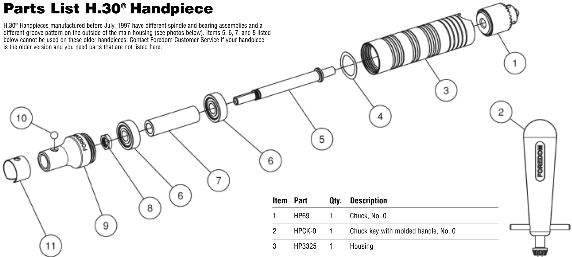
Current H.30® Handpiece
